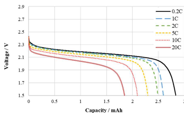
Discharge characteristics
