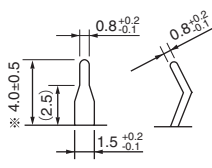
(Terminal dimensions)
