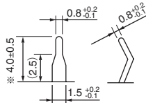
(Terminal dimensions)
